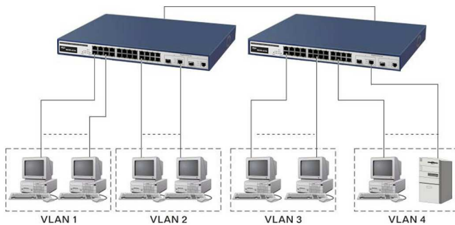
Fig. 2-5 Port-based VLAN Diagram
