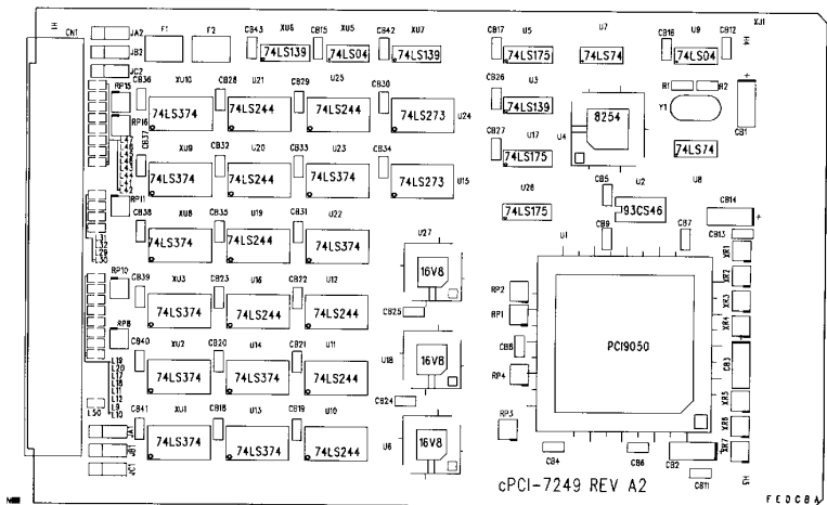
Figure 2.3.4 cPCI-7249R Layout
