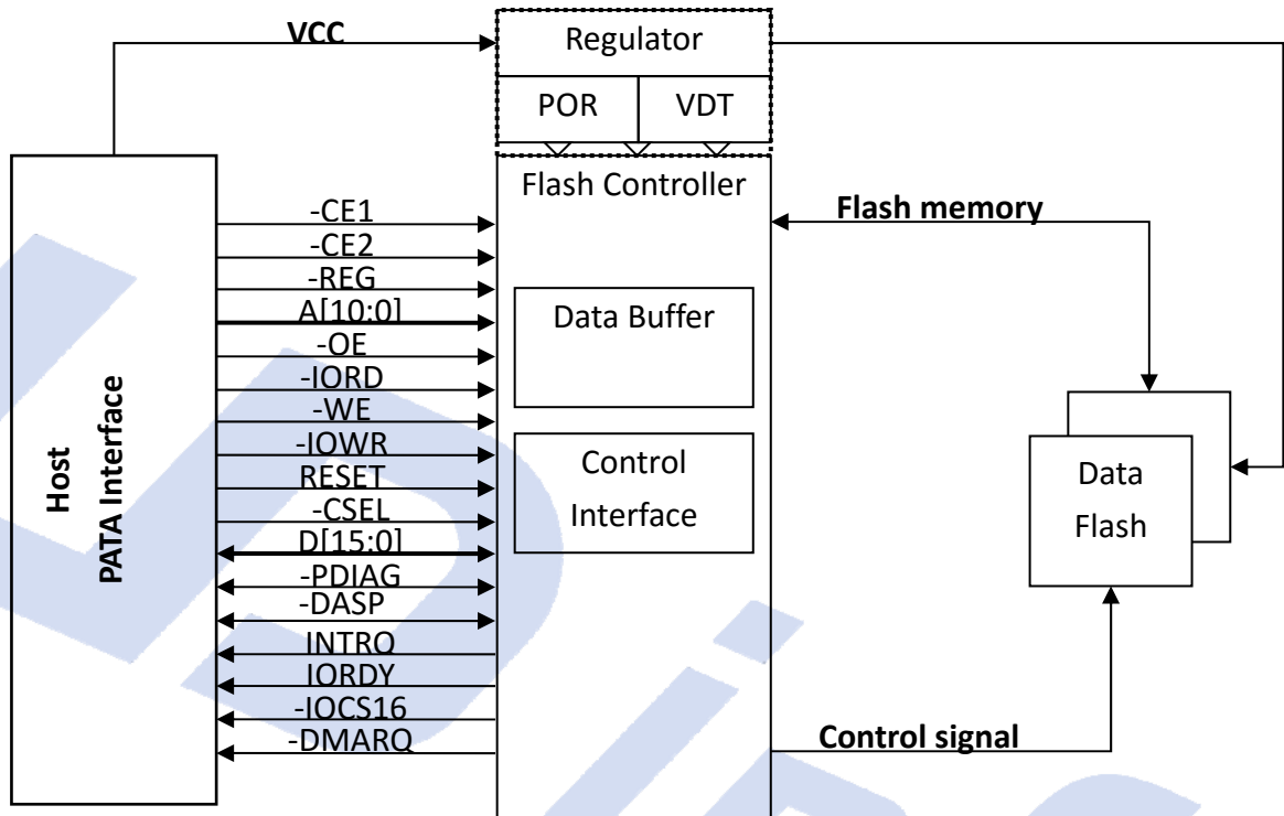
Micro Disk Module Block Diagram
