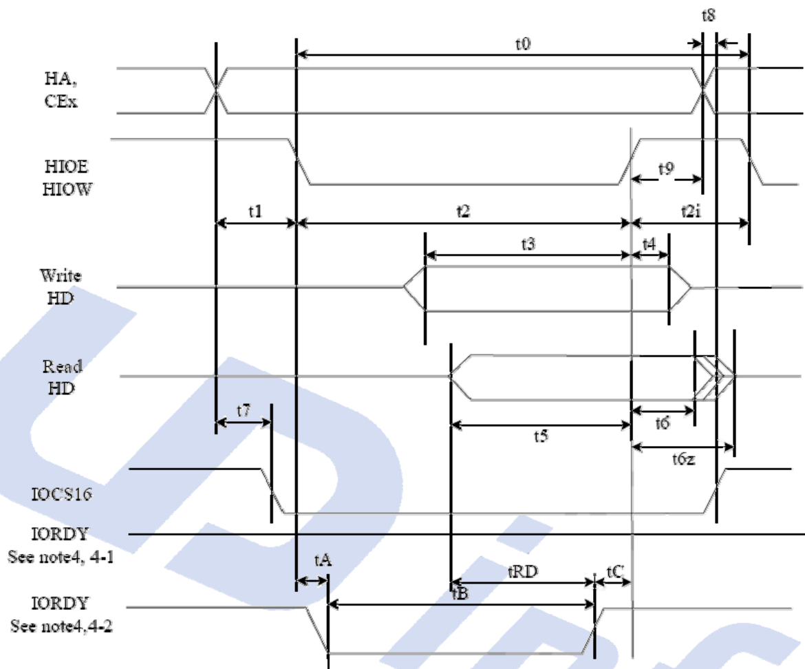
True IDE Mode Read/Write Timing Diagram
